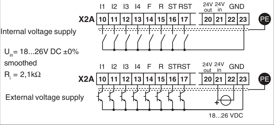
Fig. 6.3.2.b Digital inputs with NPN control (di.0 = 1)
