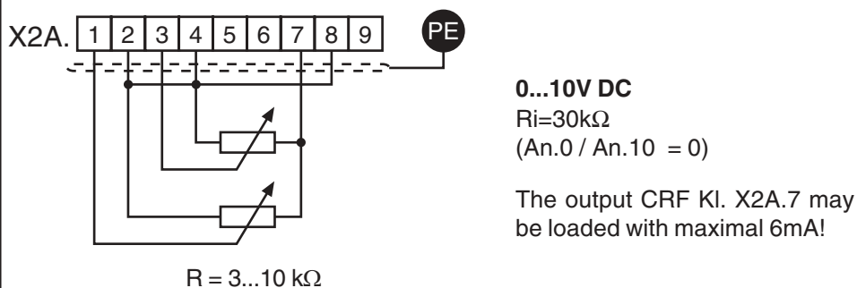
Fig. 6.2.2.b Control with potentiometer and internal reference voltage
