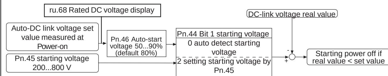
Fig. 6.9.6.a Starting the Power-Off function
