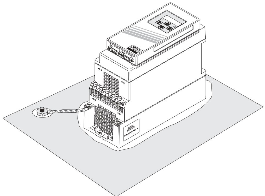
Picture 7.1.2.a Installation and connection
