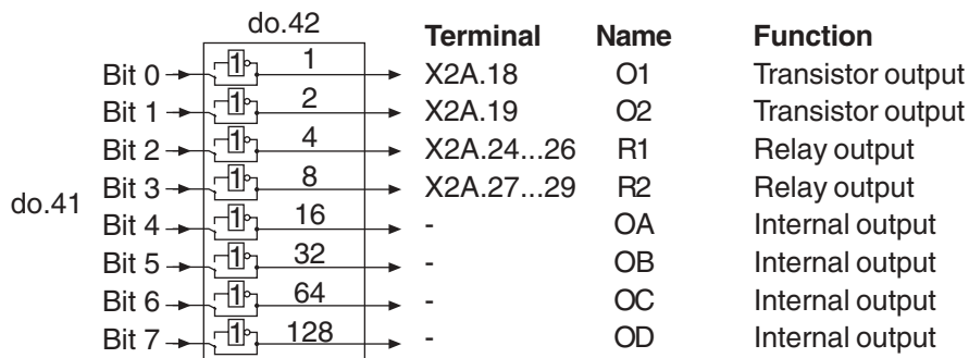
Fig. 6.3.21 Inverting the outputs
