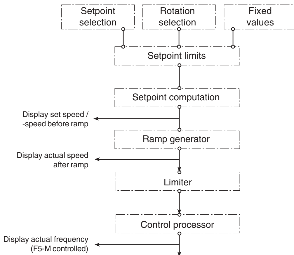
Fig. 6.4.1 Principle of set value and ramp adjustment
