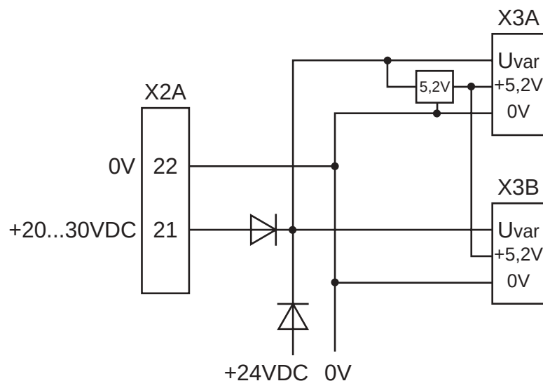
Fig. 6.10.4 Power supply
