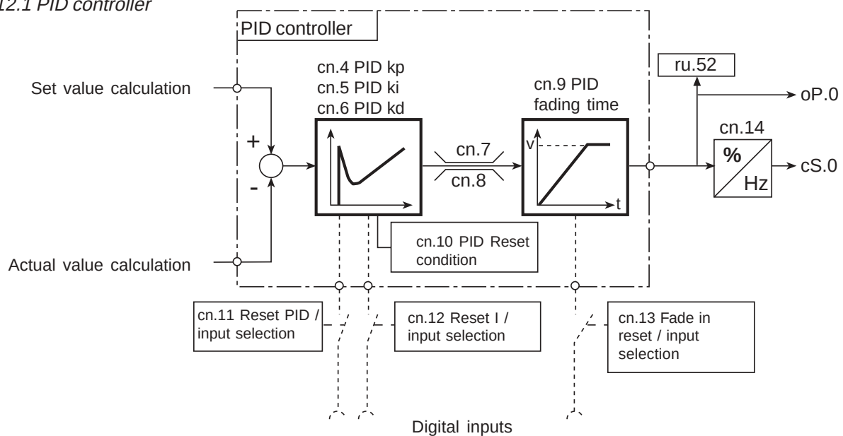
Pic. 6.12.1 PID controller
