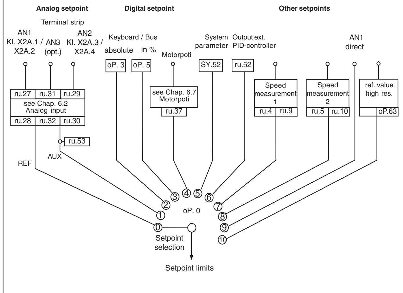
Fig. 6.4.2 Setpoint selection
