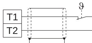
Thermo contact (NC contact)
