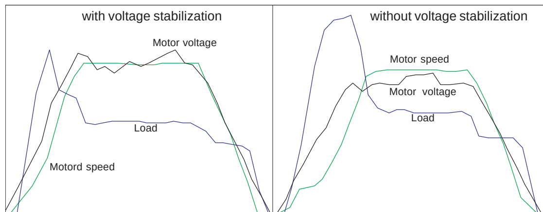
Fig. 6.5.5.b Example: Acceleration with load
