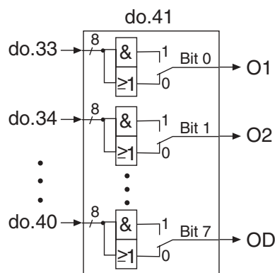
Fig. 6.3.19 Linking the switching conditions in logic step 2
