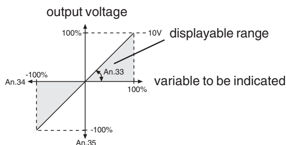
Fig. 6.2.14.a Factory setting: no Offset, Gain 1
