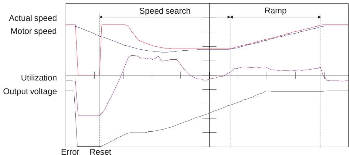
Fig. 6.7.3.c Speed search with „fast“ adjusted function
