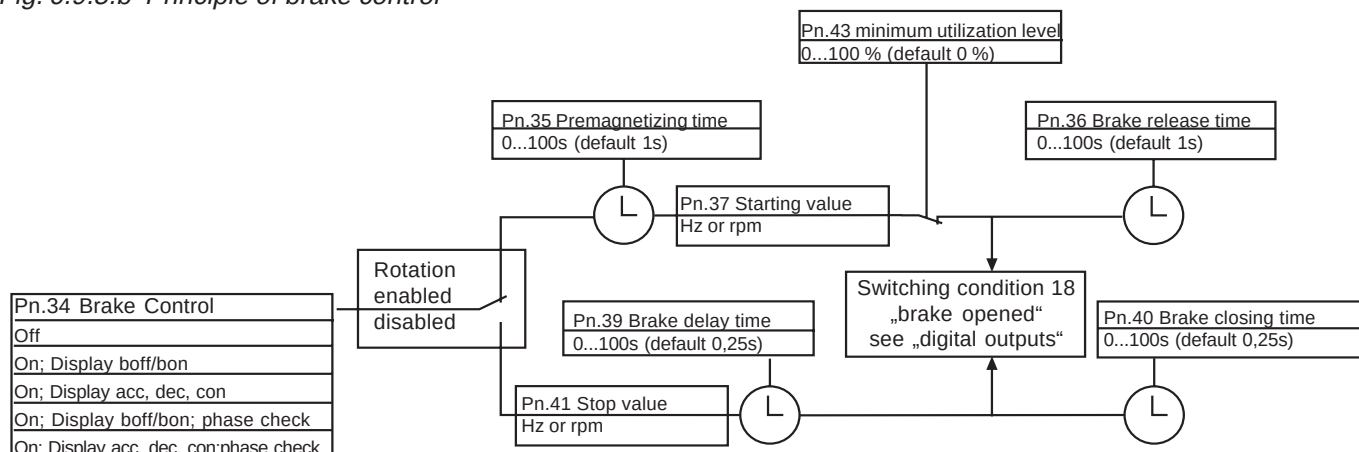
Fig. 6.9.5.b Principle of brake control
