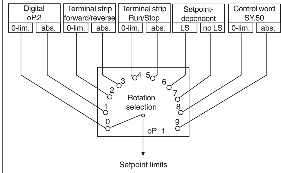
Fig. 6.4.3 Rotation selection with oP.1
