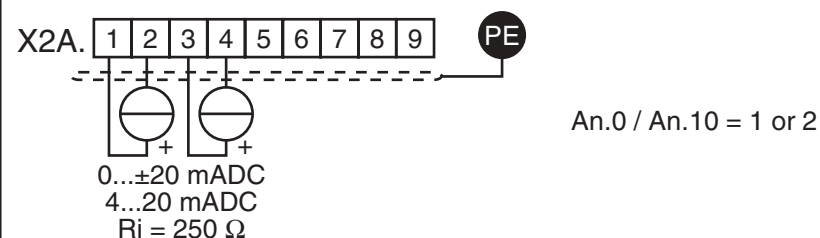
Fig. 6.2.2.c Control with current signal
