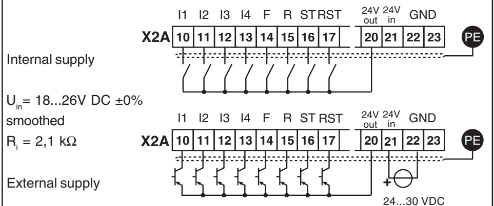
Fig. 6.3.2.a Digital inputs with PNP control (di.0 = 0)
