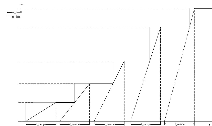
Fig. 6.4.9.a Forward acceleration with constant ramp time
