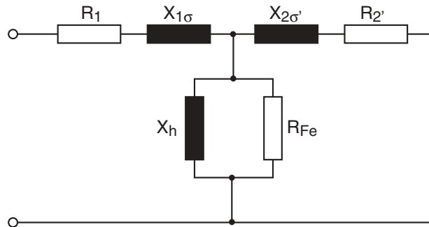
Fig. 6.6.3 Equivalent circuit diagram of a motor in phase quantities
