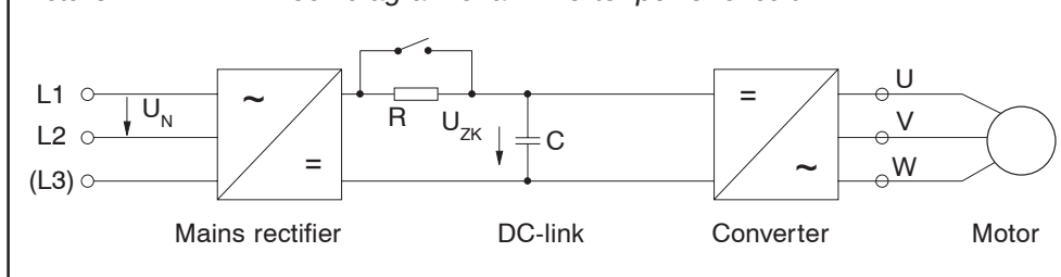
Picture 2.1.2 Block diagram of an inverter power circuit
