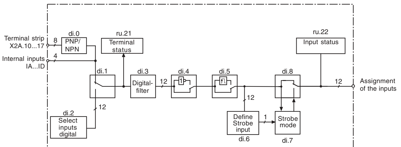
Fig. 6.3.1 Principle of digital inputs
