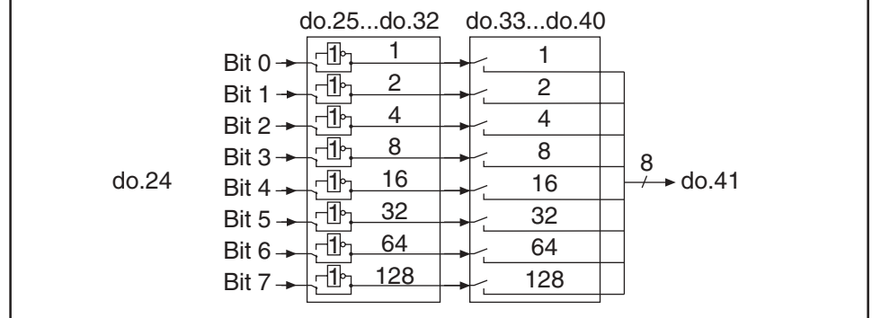
Fig. 6.3.18 Inversion and selection of switching conditions from step 1
