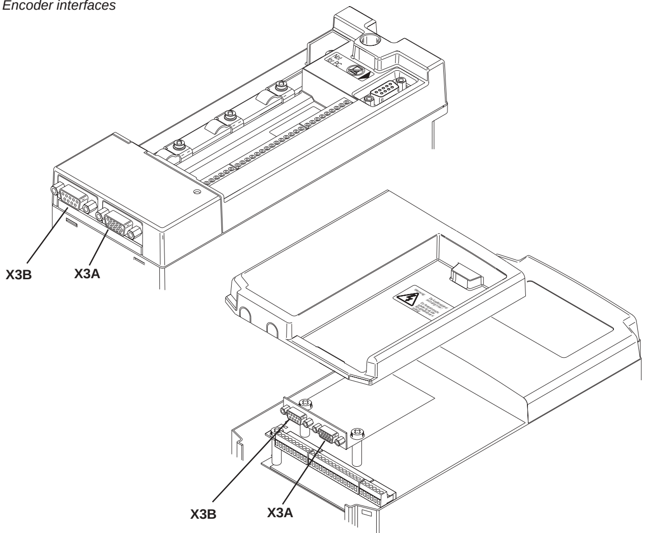
6.10.1 Encoder interfaces
