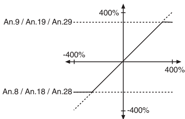
Fig. 6.2.8 Limiting of the analog signal
