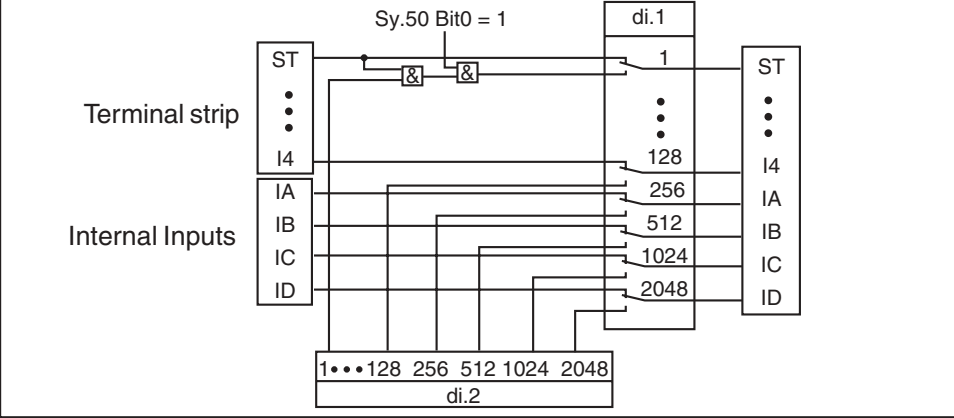
Fig. 6.3.3 Digital inputs controlled by Software (di.1/di.2)
