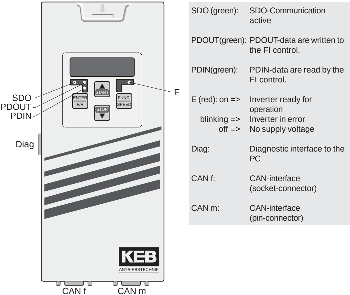
Fig. 11.1.7 CanOpen Operator
