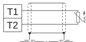
Temperature sensor (PTC) 1650Ω...4kΩ tripping resistance 750Ω...1650Ω reset resistance
