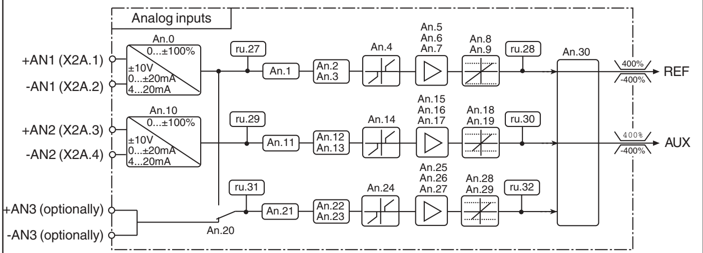
Fig. 6.2.1 Principle of the analog inputs
