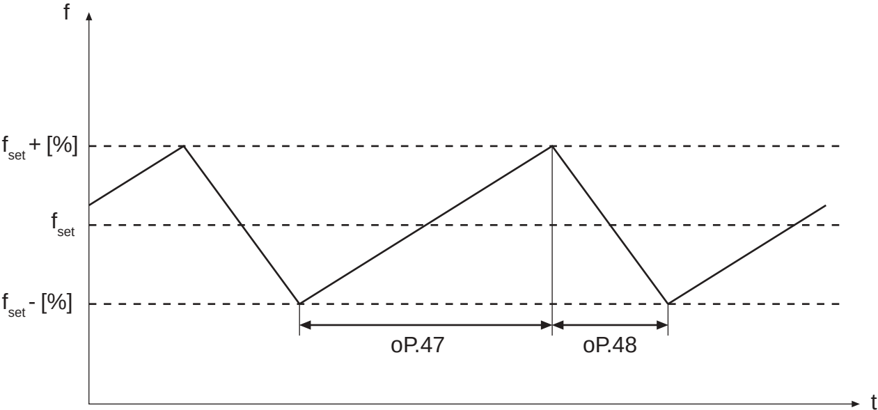
6.9.7.b Acceleration and deceleration times of the wobbel generator
