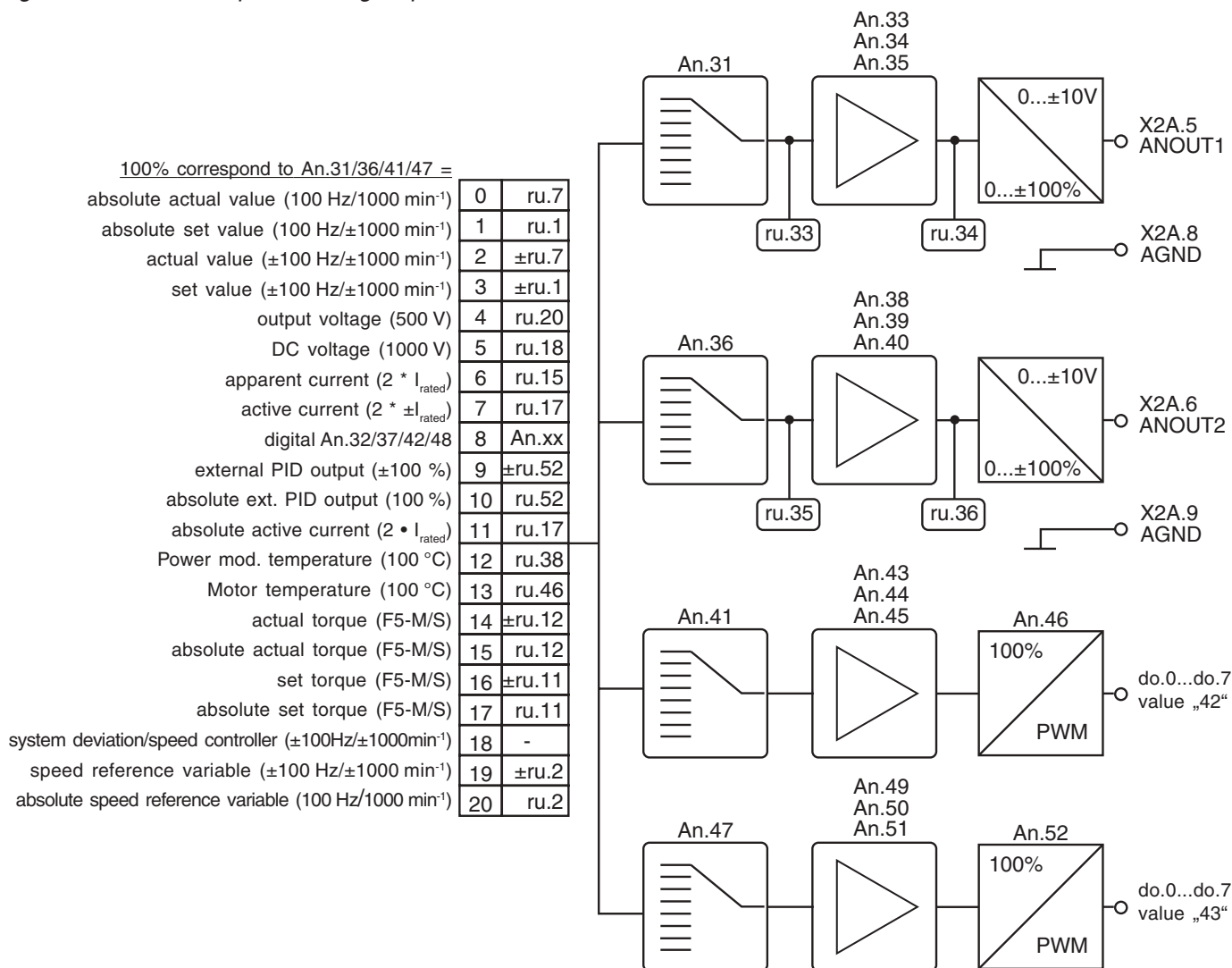
Fig. 6.2.10 Principle of analog output
