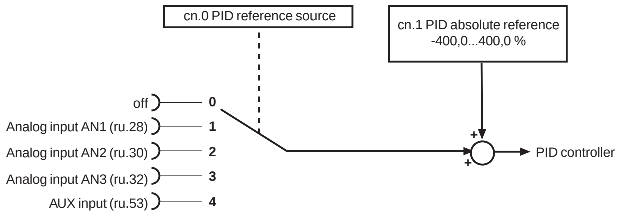
Pic. 6.12.2 PID controller set value
