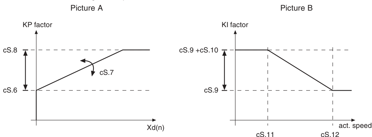
Fig. 6.6.11 Mode of functioning of the speed controller
