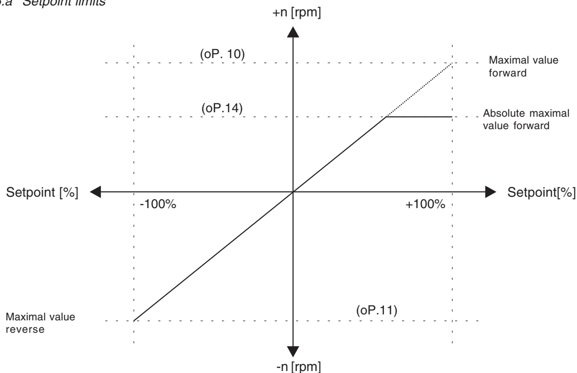
Fig. 6.4.5.a Setpoint limits
