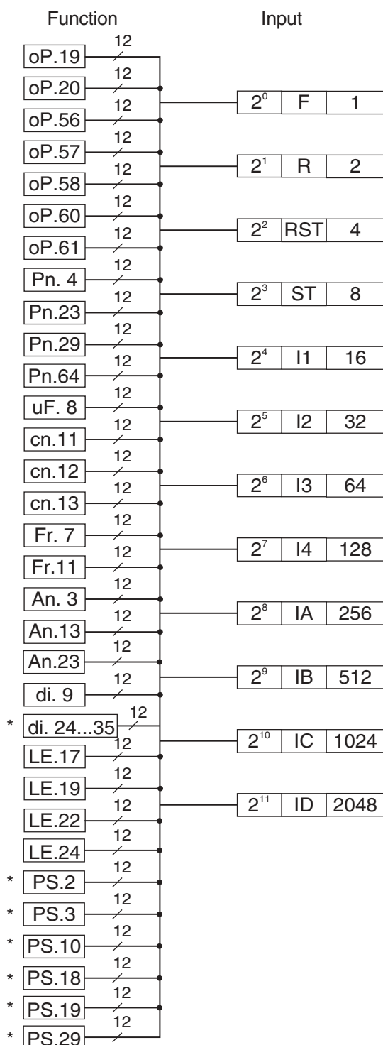
Fig. 6.3.11b Function-related assignment
