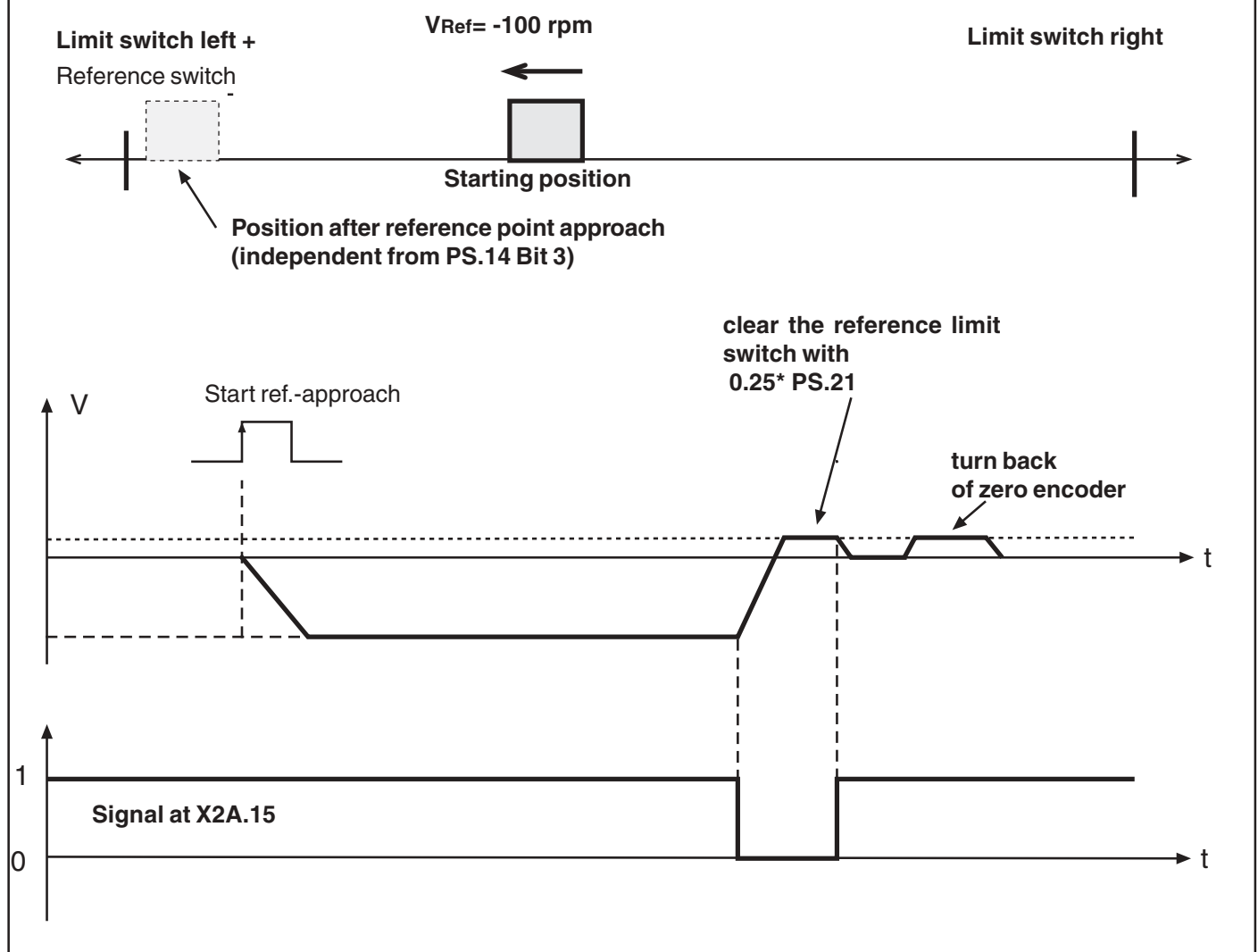
Pic. 6.11.6.a Reference point approach example 1
