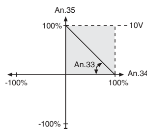
Fig. 6.2.14.b Inverting the analog output
