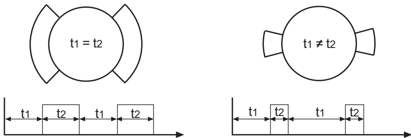
Symmetrical and asymmetrical cam arrangement
