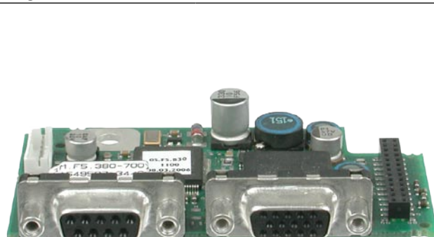
Figure 2: Encoder interface 1MF5280-7007
